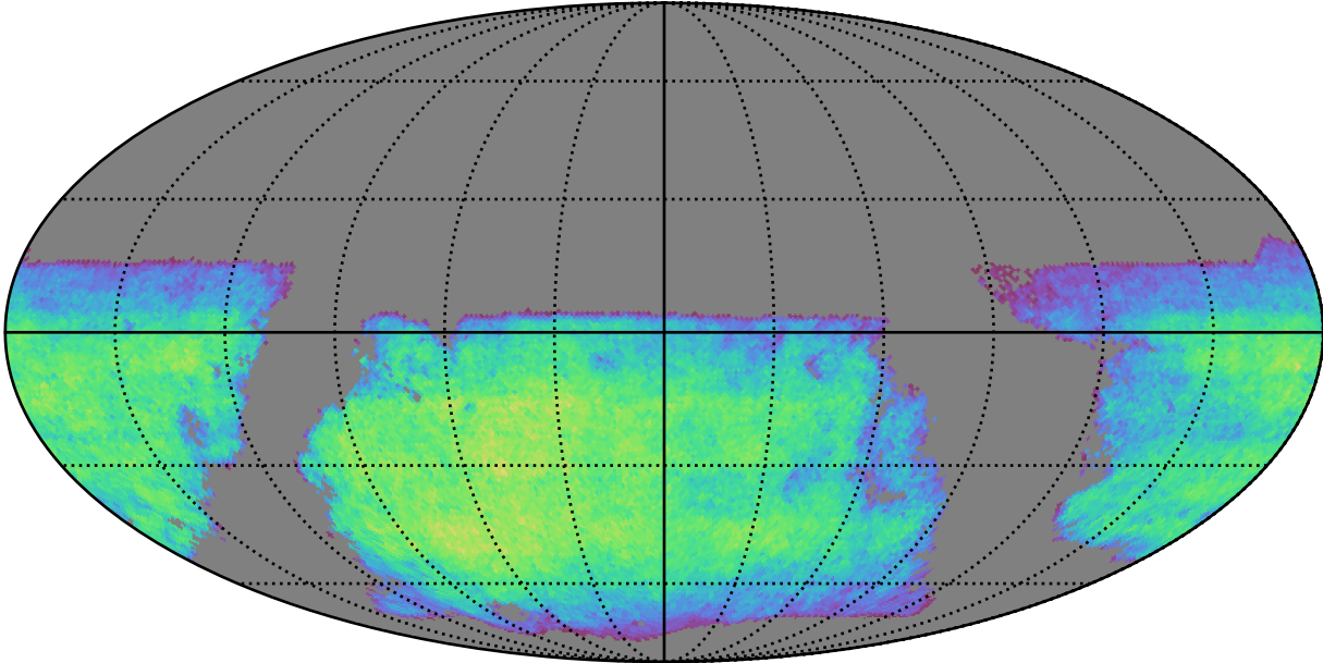
early_ss_template_fpextra1.5_v3.4_10yrs i band non-DD year 6: ExgalM5WithCuts
