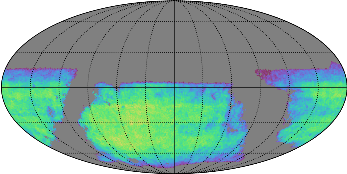
early_ss_template_fpextra1.5_v3.4_10yrs i band non-DD year 4: ExgalM5WithCuts
