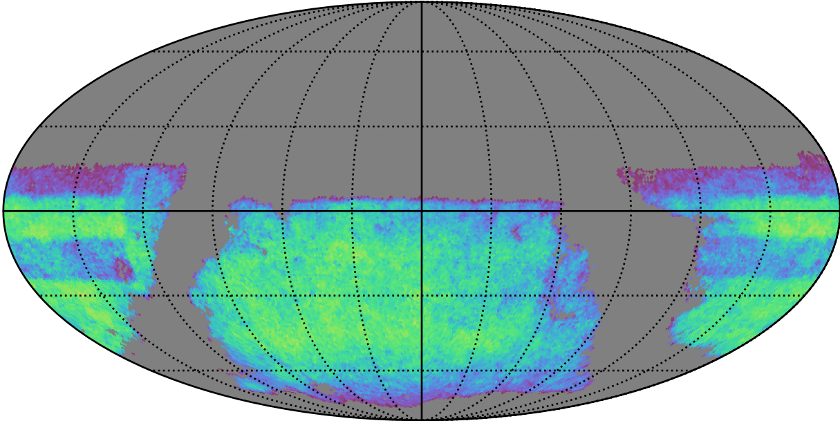
early_ss_template_fpextra1.5_v3.4_10yrs i band non-DD year 2: ExgalM5WithCuts
