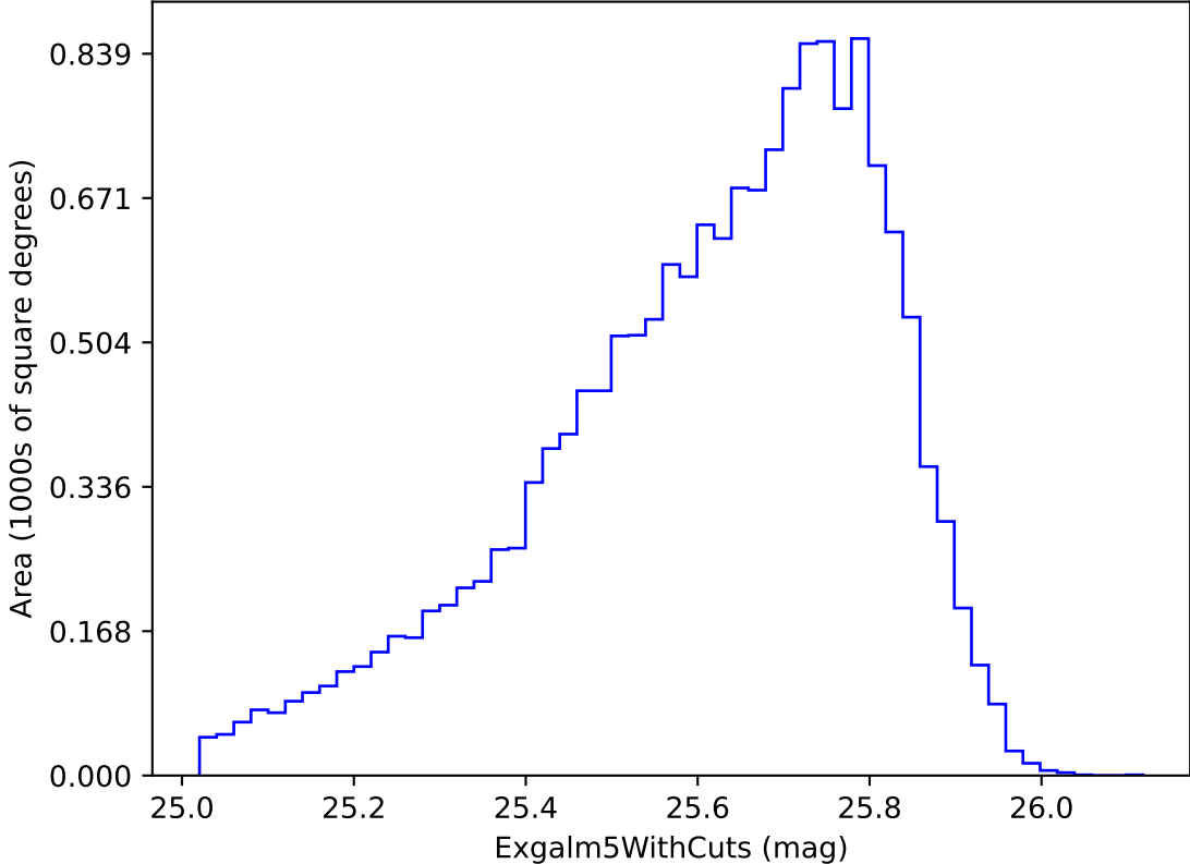
early_ss_template_fpextra1.5_v3.4_10yrs i band non-DD year 2: ExgalM5WithCuts
