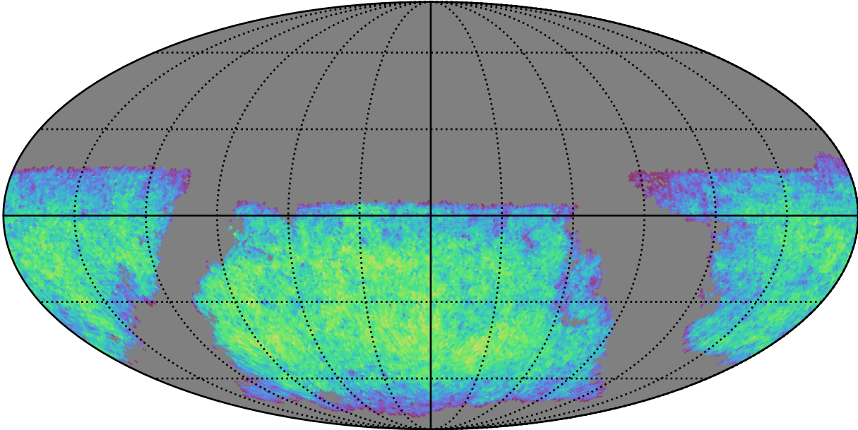
early_ss_template_fpextra1.5_v3.4_10yrs i band non-DD year 1: ExgalM5WithCuts
