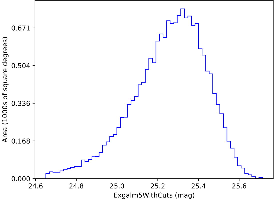
early_ss_template_fpextra1.5_v3.4_10yrs i band non-DD year 1: ExgalM5WithCuts
