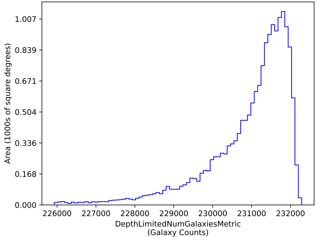
early_ss_template_fpextra1.5_v3.4_10yrs i band galaxies non-DD: DepthLimitedNumGalaxiesMetric
