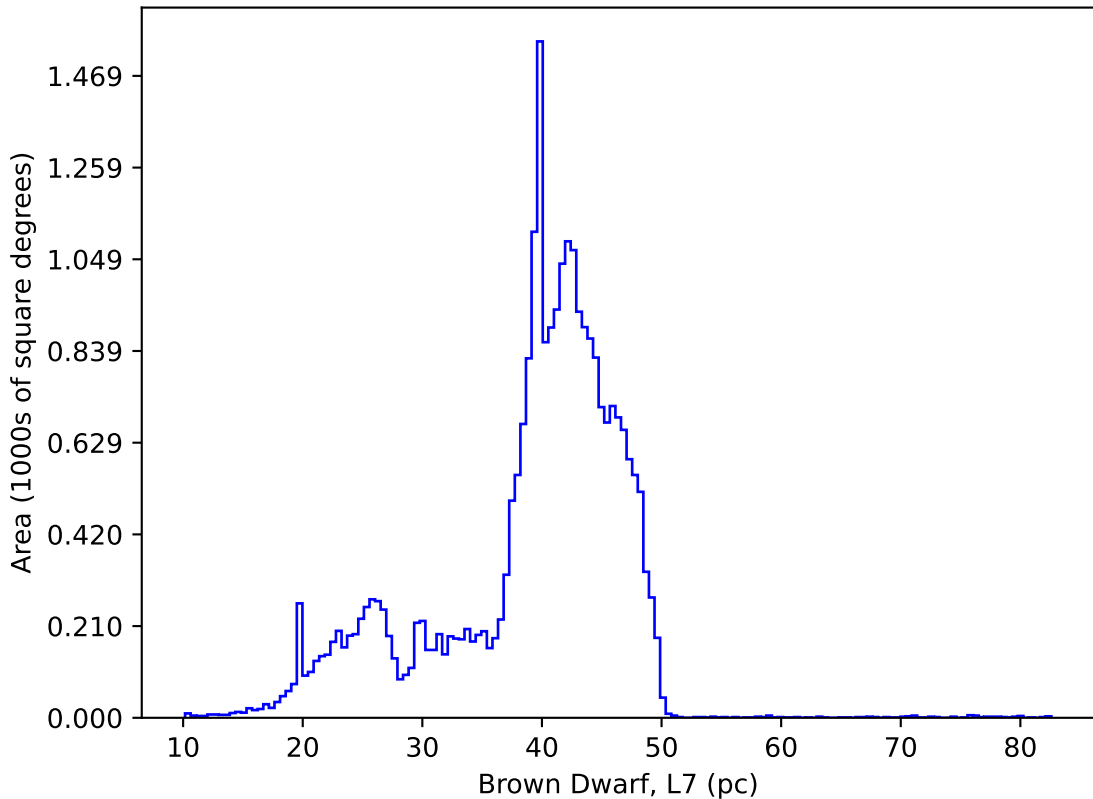
early_ss_template_fpextra1.5_v3.4_10yrs : Brown Dwarf, L7
