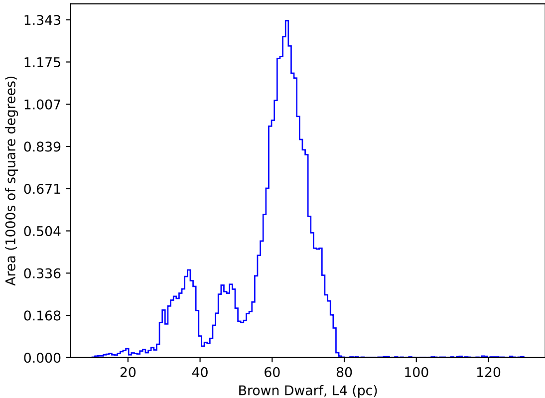
early_ss_template_fpextra1.5_v3.4_10yrs : Brown Dwarf, L4
