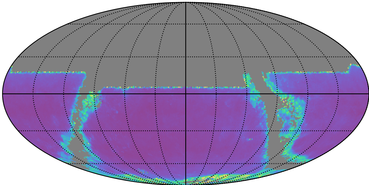
early_ss_template_fpextra1.5_v3.4_10yrs y band: AGN SF_uncert
