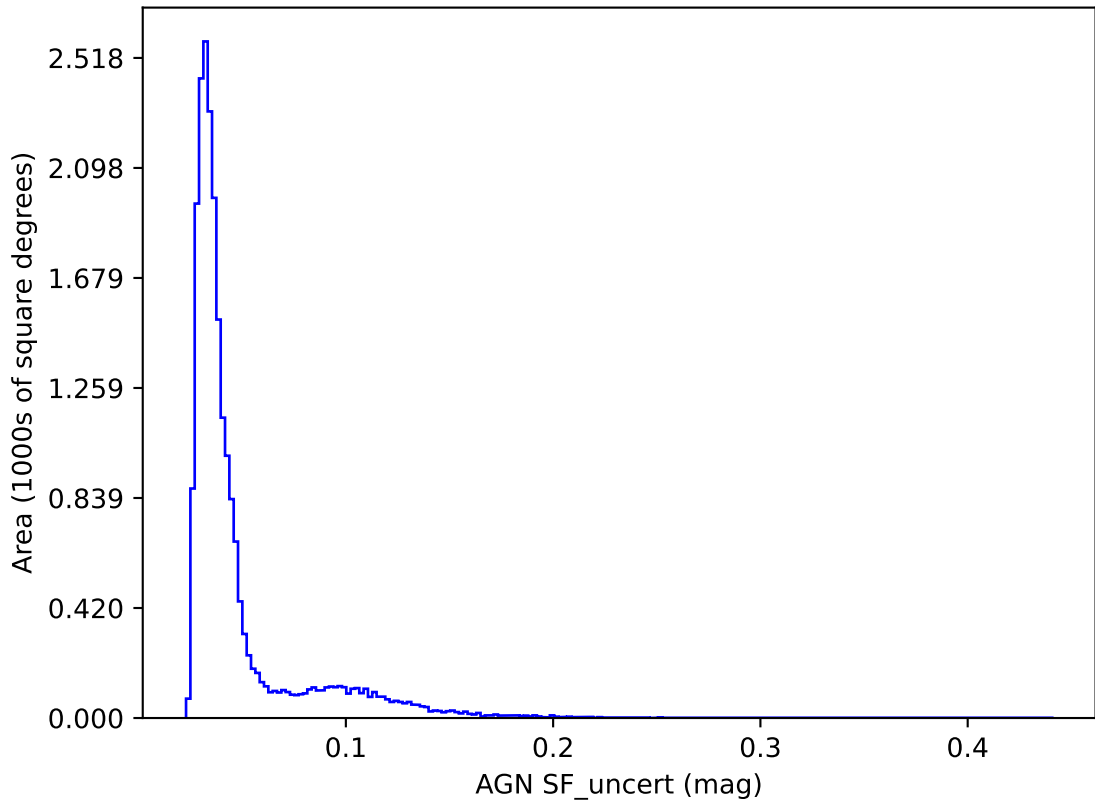
early_ss_template_fpextra1.5_v3.4_10yrs y band: AGN SF_uncert
