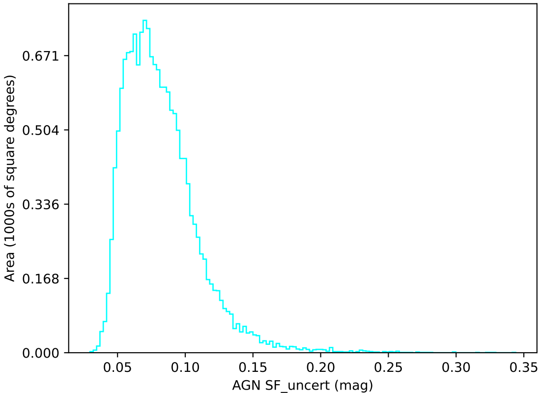
early_ss_template_fpextra1.5_v3.4_10yrs u band: AGN SF_uncert
