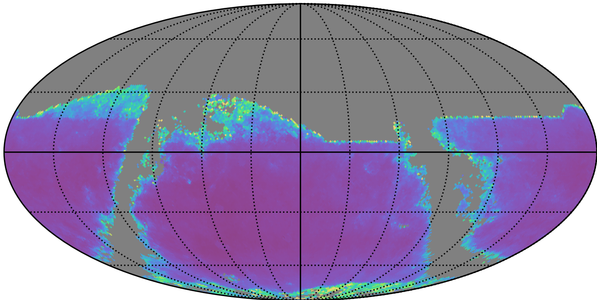
early_ss_template_fpextra1.5_v3.4_10yrs r band: AGN SF_uncert
