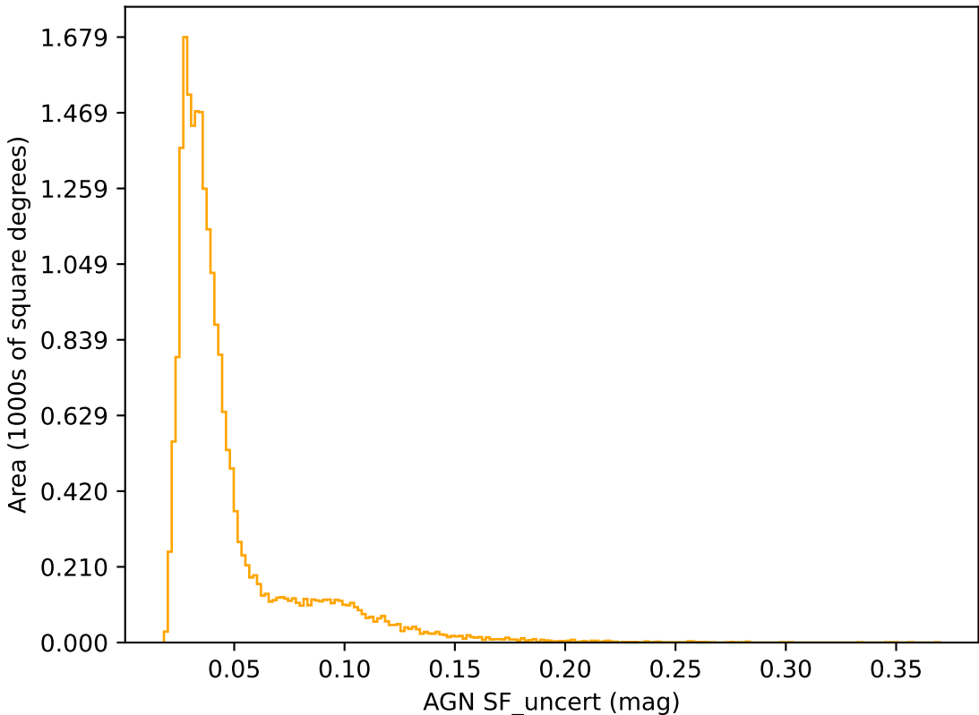
early_ss_template_fpextra1.5_v3.4_10yrs r band: AGN SF_uncert
