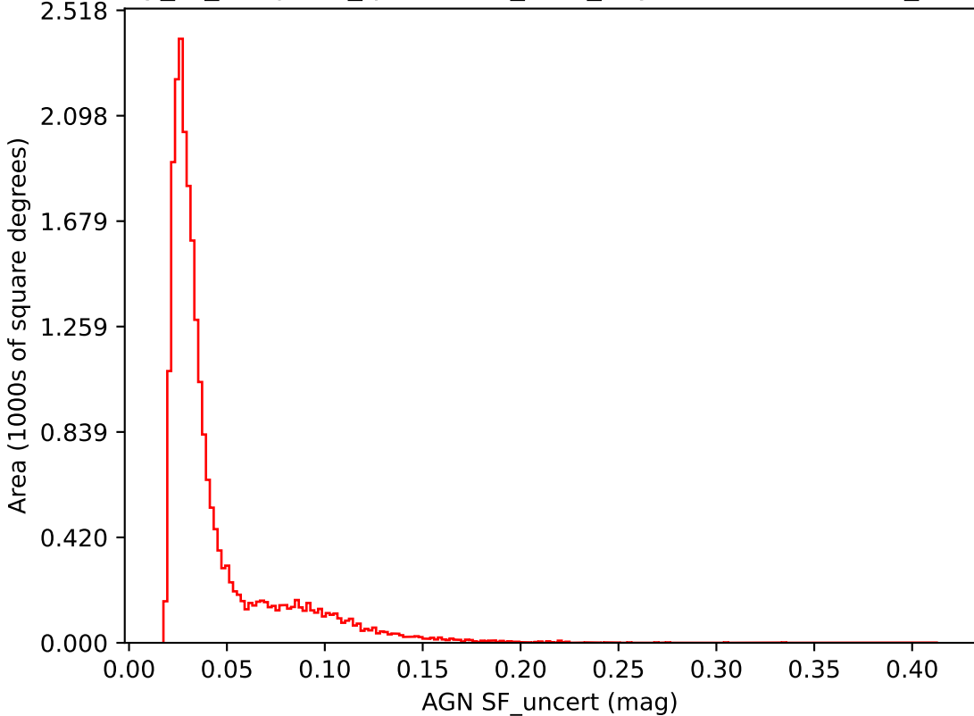
early_ss_template_fpextra1.5_v3.4_10yrs i band: AGN SF_uncert
