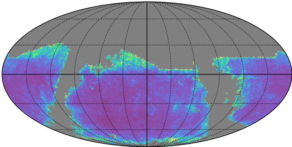
early_ss_template_fpextra1.5_v3.4_10yrs g band: AGN SF_uncert
