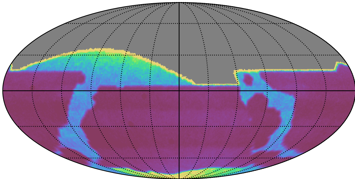
early_ss_template_fpextra1.5_v3.4_10yrs : properMotion
