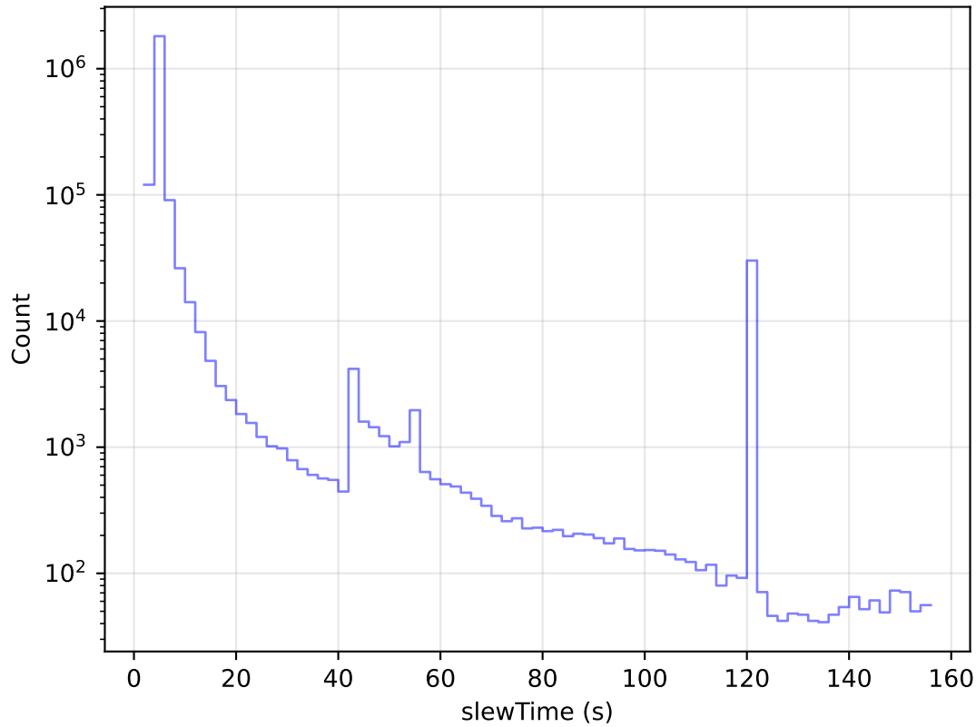
early_ss_template_fpextra1.5_v3.4_10yrs All visits: Slew Time Histogram
