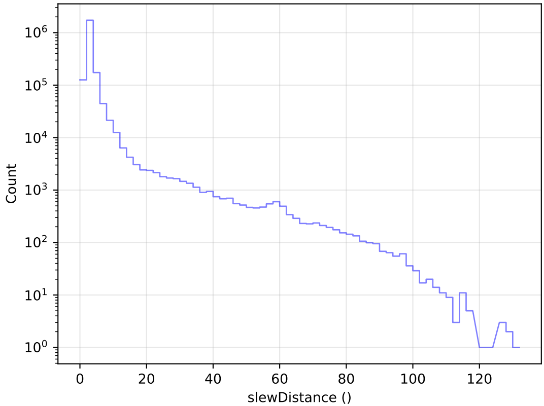
early_ss_template_fpextra1.5_v3.4_10yrs All visits: Slew Distance Histogram
