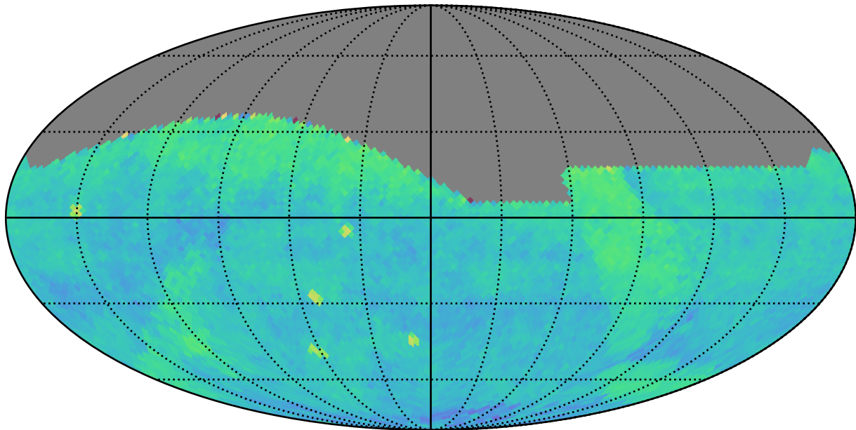
early_ss_template_fpextra1.5_v3.4_10yrs (g or r or i): PairFraction
