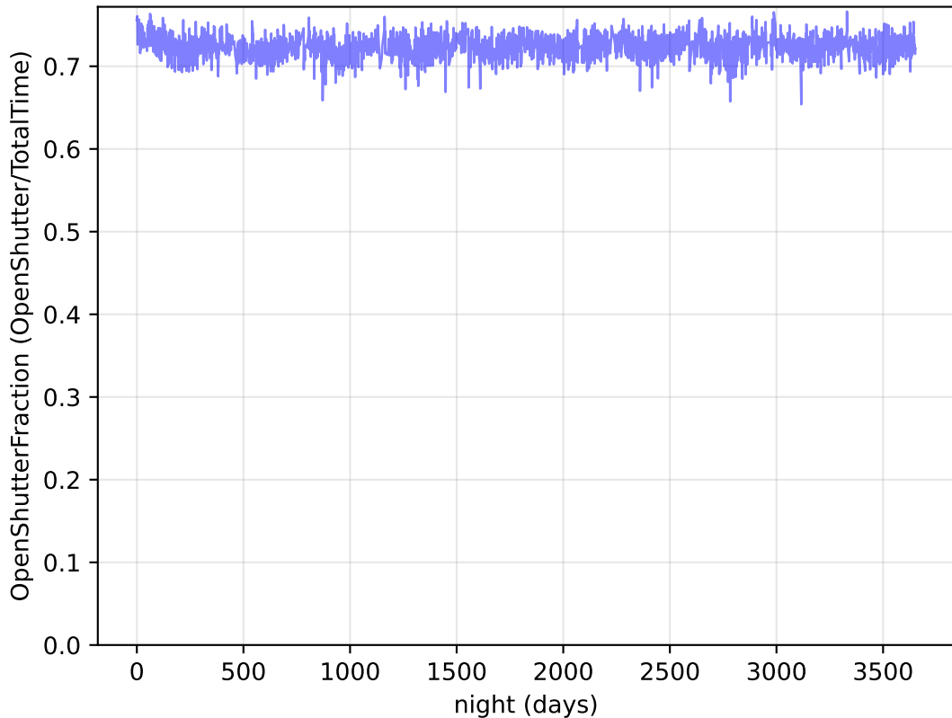
early_ss_template_fpextra1.5_v3.4_10yrs : OpenShutterFraction
