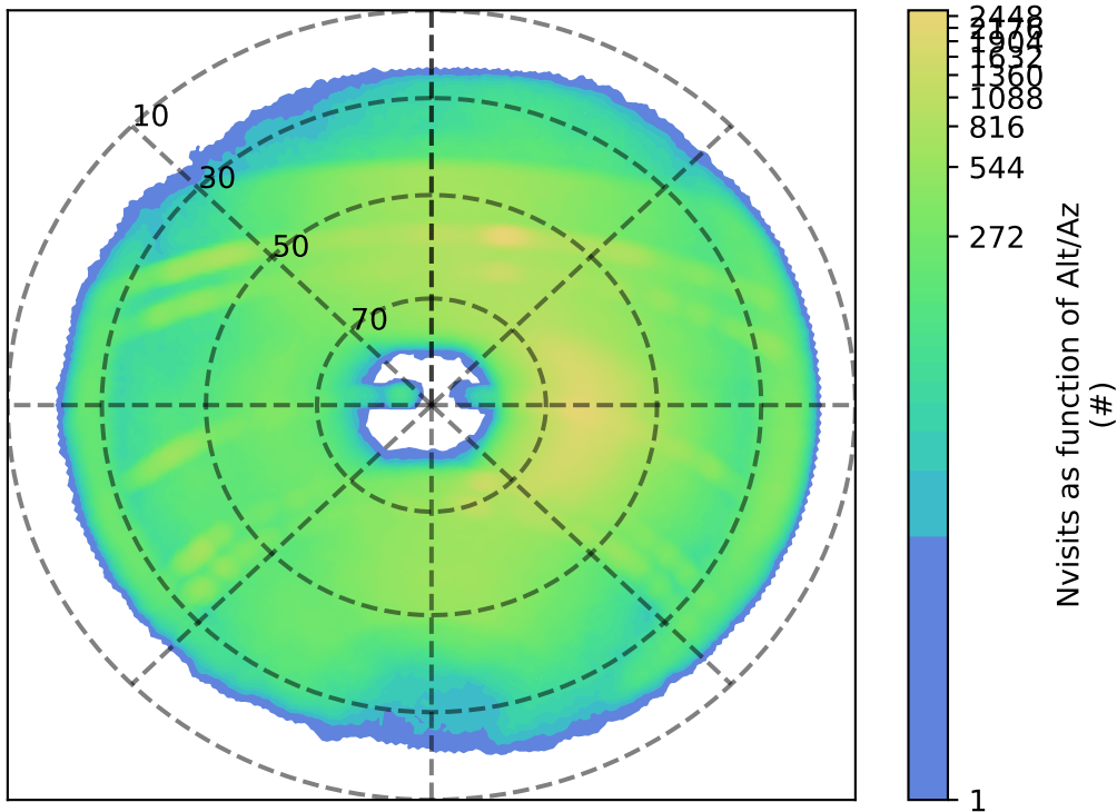
early_ss_template_fpextra1.5_v3.4_10yrs z: Nvisits as function of Alt/Az
