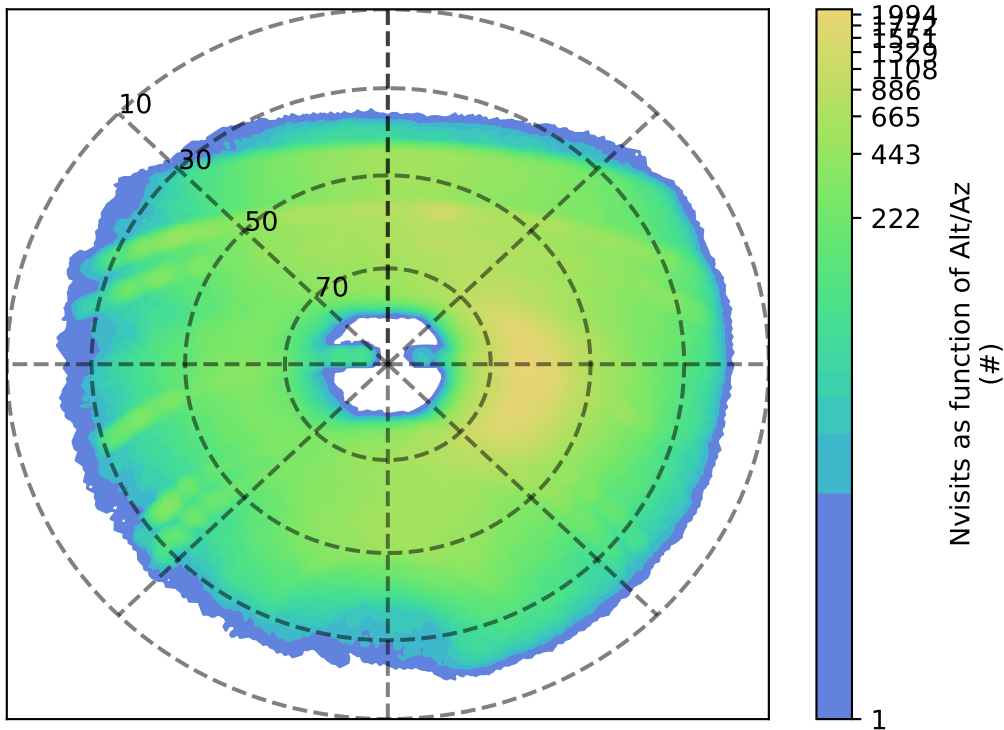
early_ss_template_fpextra1.5_v3.4_10yrs y: Nvisits as function of Alt/Az
