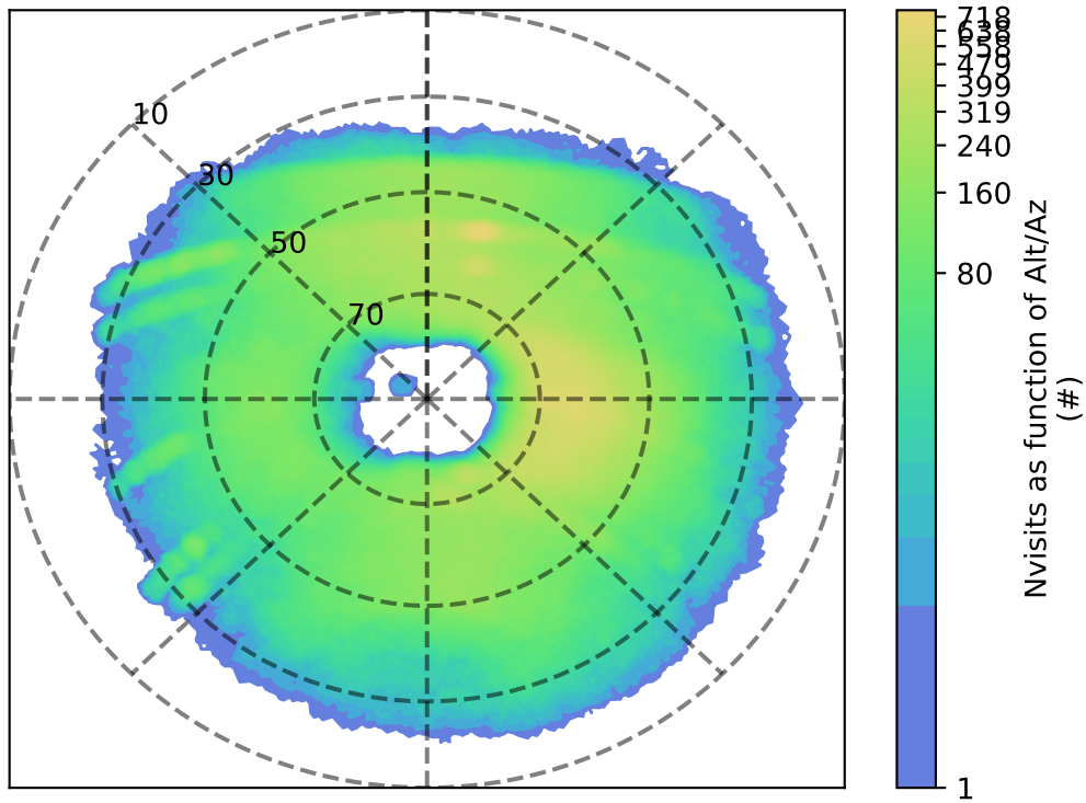
early_ss_template_fpextra1.5_v3.4_10yrs u: Nvisits as function of Alt/Az
