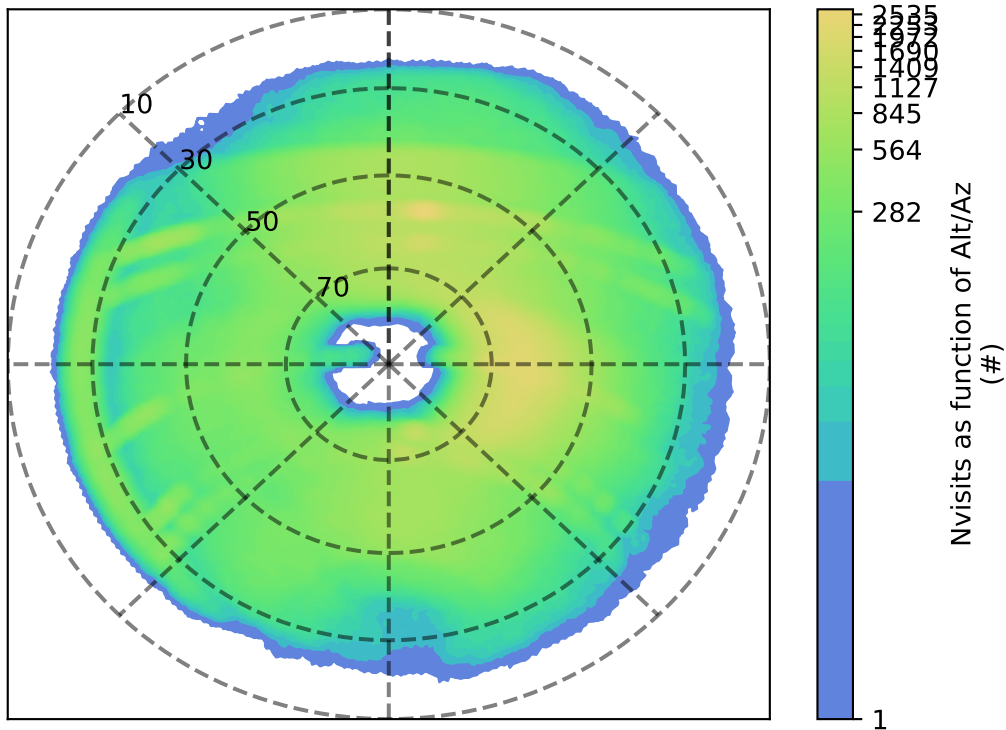
early_ss_template_fpextra1.5_v3.4_10yrs r: Nvisits as function of Alt/Az
