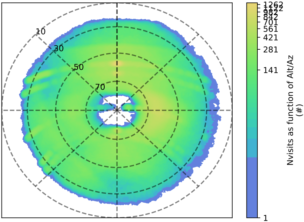
early_ss_template_fpextra1.5_v3.4_10yrs g: Nvisits as function of Alt/Az
