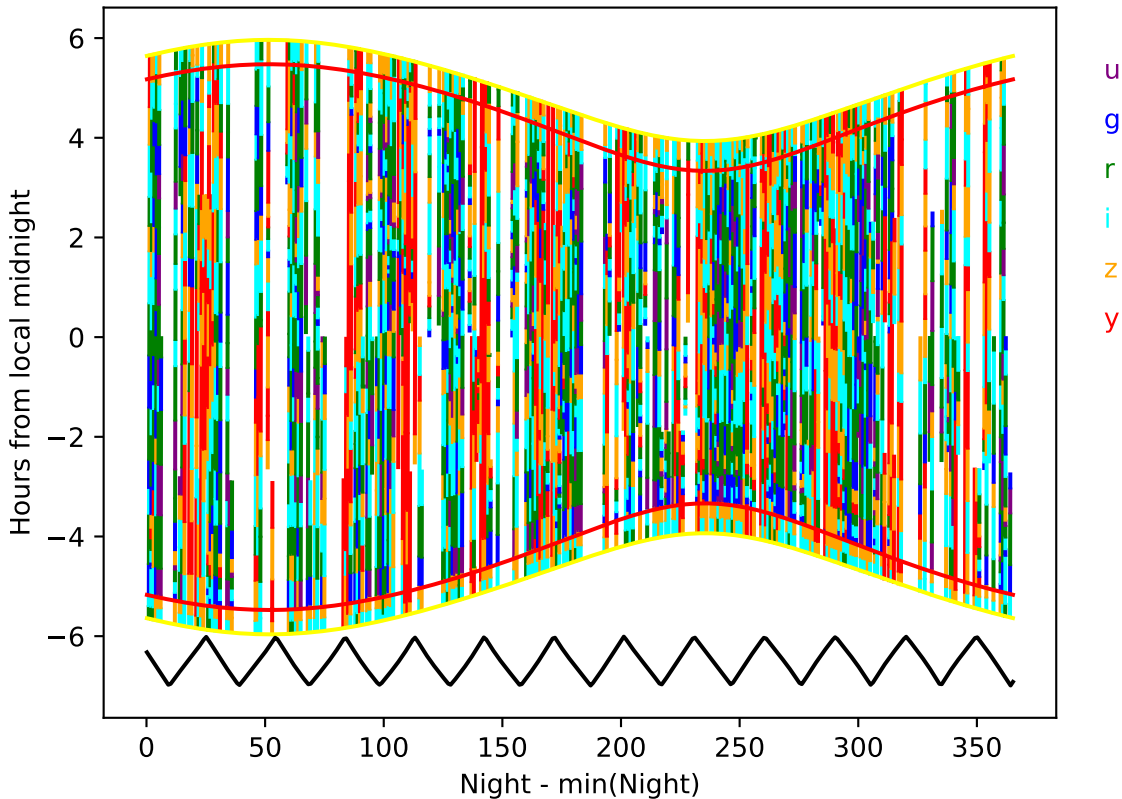
early_ss_template_fpextra1.5_v3.4_10yrs year 7-8: Hourglass
