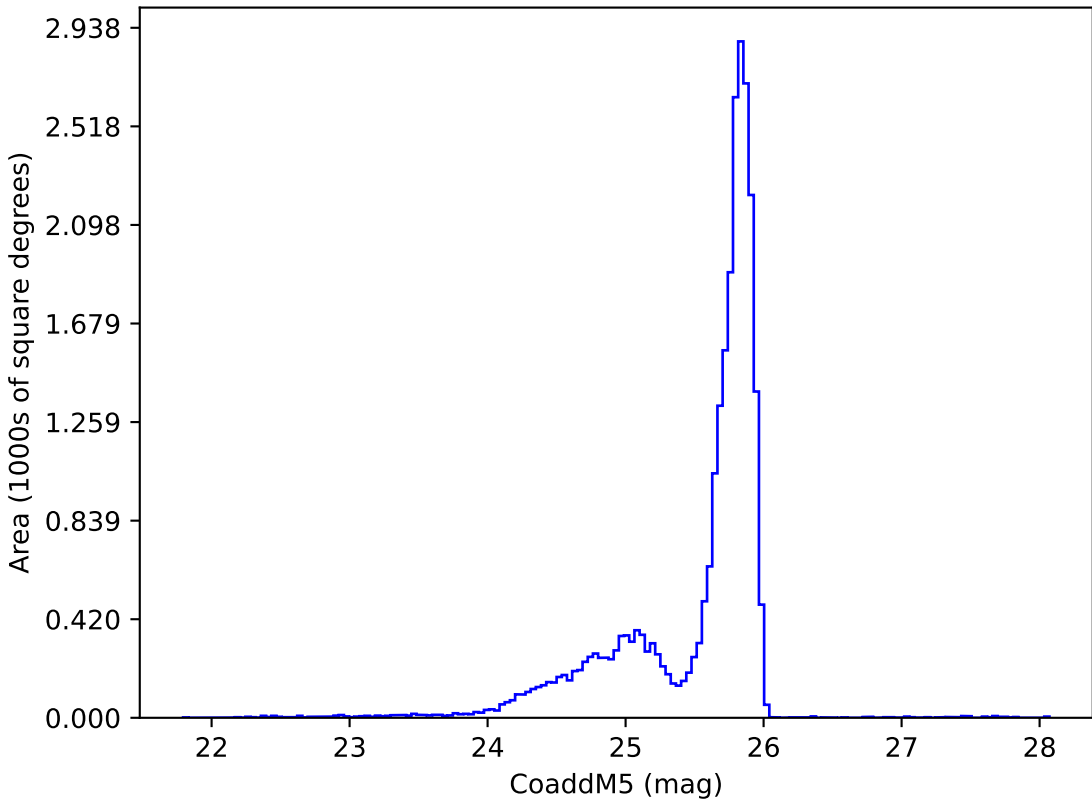
early_ss_template_fpextra1.5_v3.4_10yrs z: CoaddM5
