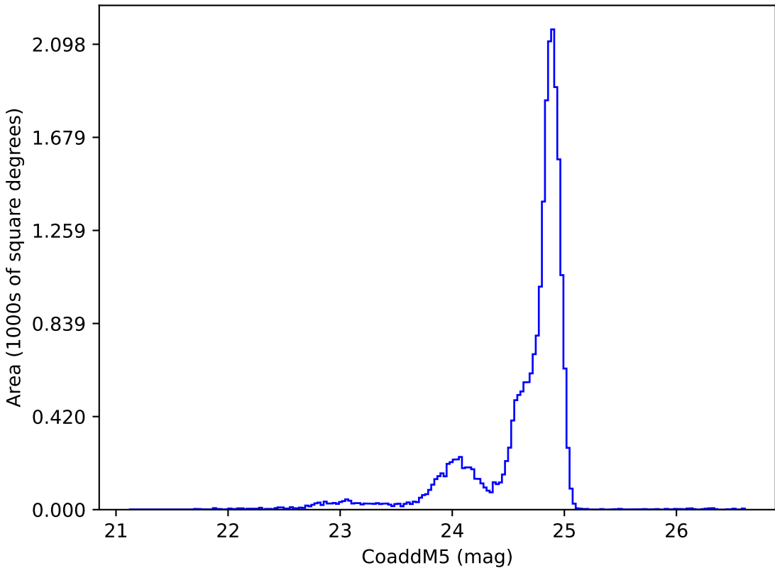
early_ss_template_fpextra1.5_v3.4_10yrs y: CoaddM5
