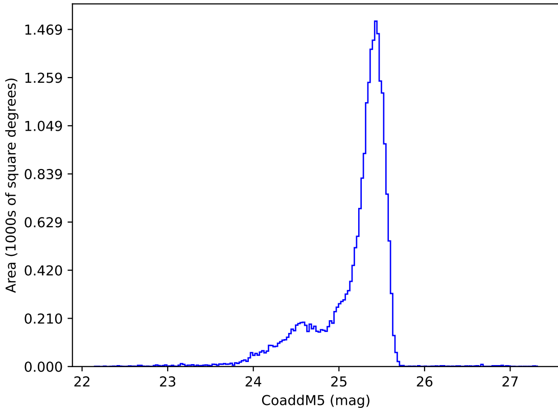
early_ss_template_fpextra1.5_v3.4_10yrs u: CoaddM5
