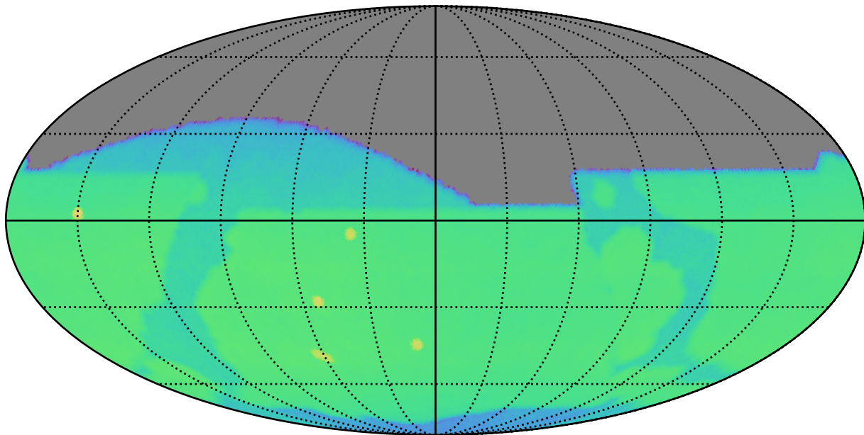
early_ss_template_fpextra1.5_v3.4_10yrs r: CoaddM5
