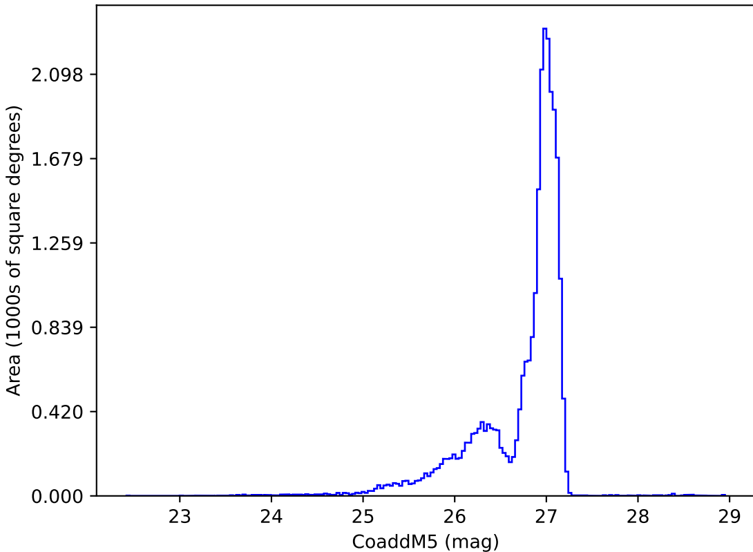
early_ss_template_fpextra1.5_v3.4_10yrs r: CoaddM5
