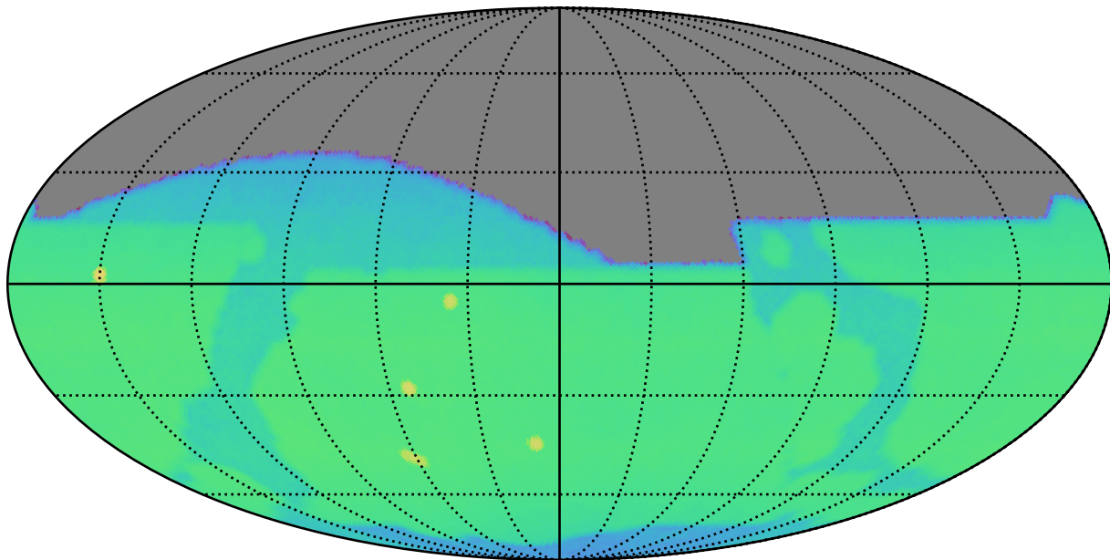
early_ss_template_fpextra1.5_v3.4_10yrs i: CoaddM5
