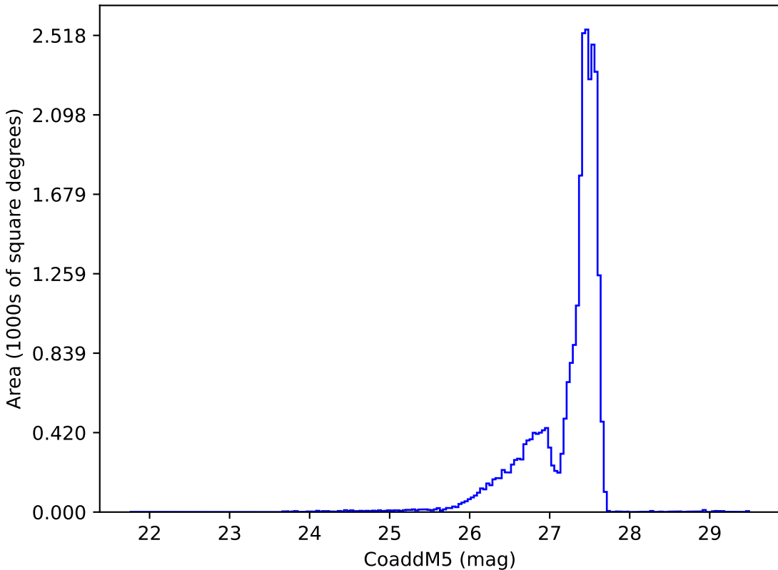
early_ss_template_fpextra1.5_v3.4_10yrs : CoaddM5
