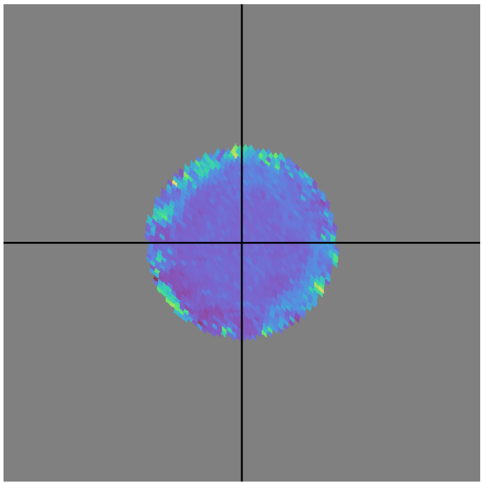
early_ss_template_fpextra1.5_v3.4_10yrs DD:ELAISS1 g band: Structure Function Uncert
