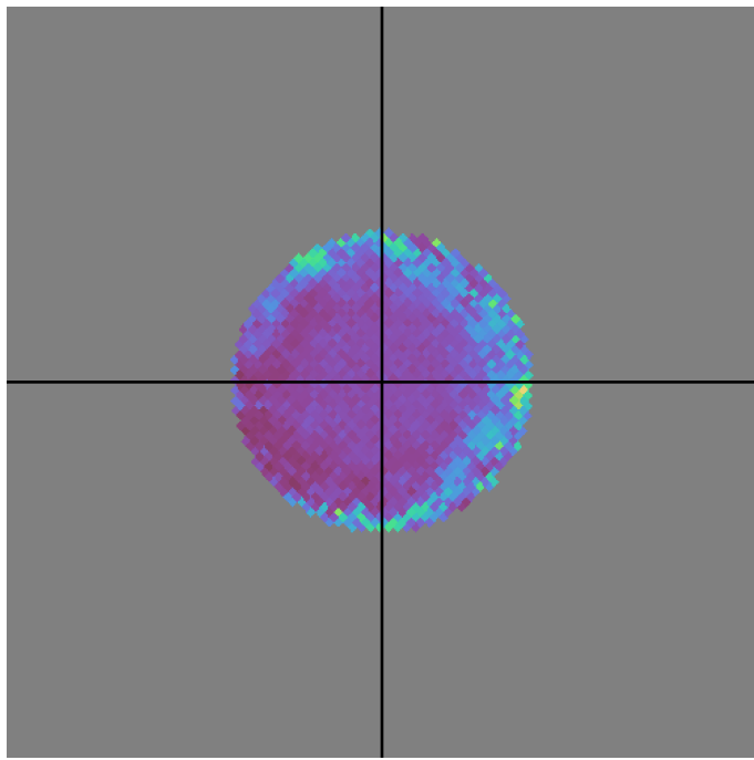
early_ss_template_fpextra1.5_v3.4_10yrs DD:ECDFS g band: Structure Function Uncert
