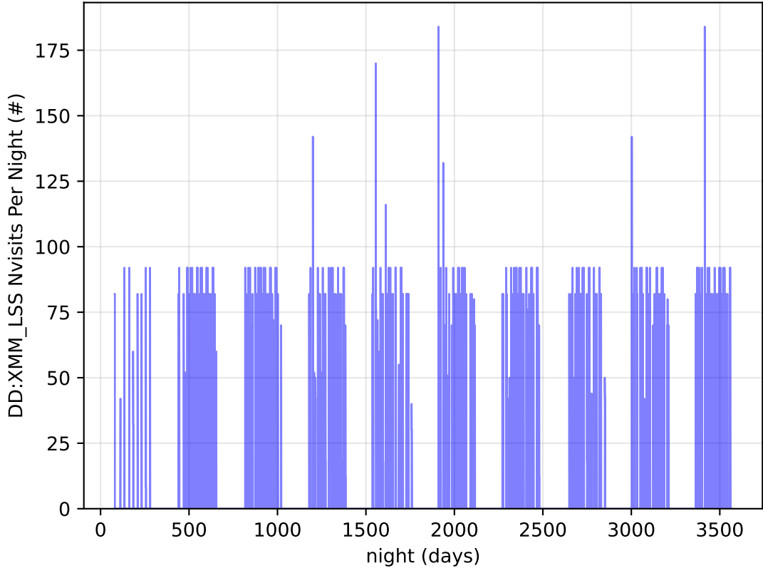
early_ss_template_fpextra1.5_v3.4_10yrs all bands: DD:XMM_LSS Nvisits Per Night
