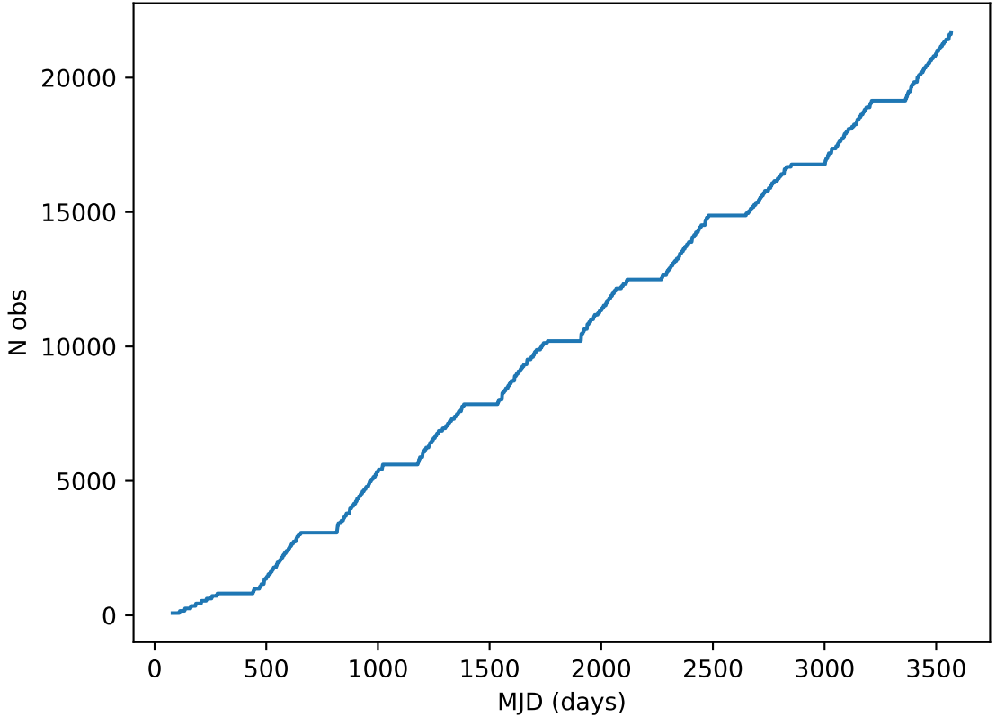
early_ss_template_fpextra1.5_v3.4_10yrs all bands: DD:XMM_LSS Cumulative NVisits
