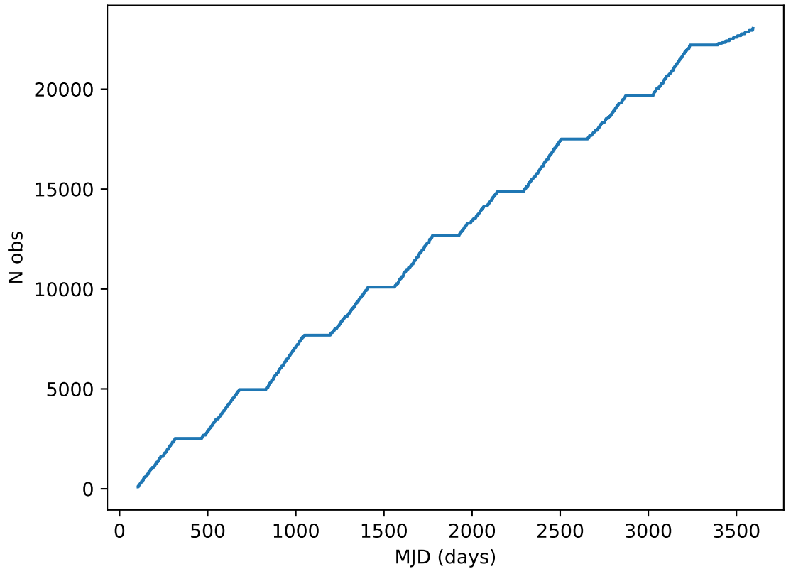
early_ss_template_fpextra1.5_v3.4_10yrs all bands: DD:EDFS Cumulative NVisits
