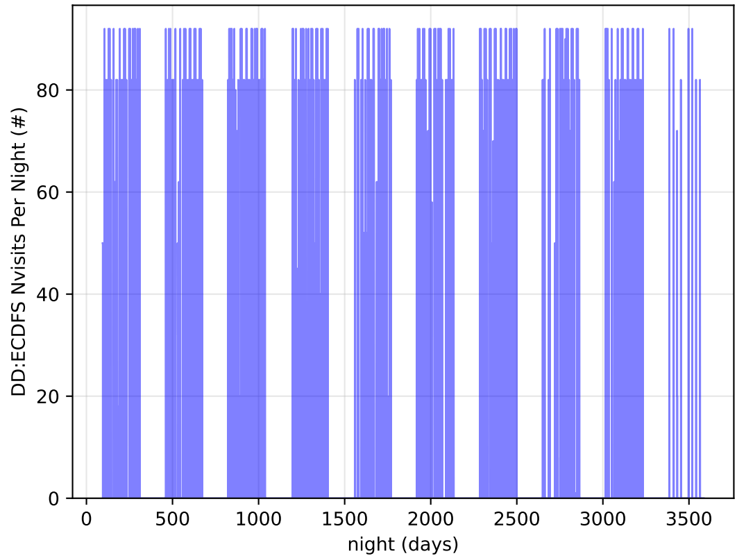
early_ss_template_fpextra1.5_v3.4_10yrs all bands: DD:ECDFS Nvisits Per Night
