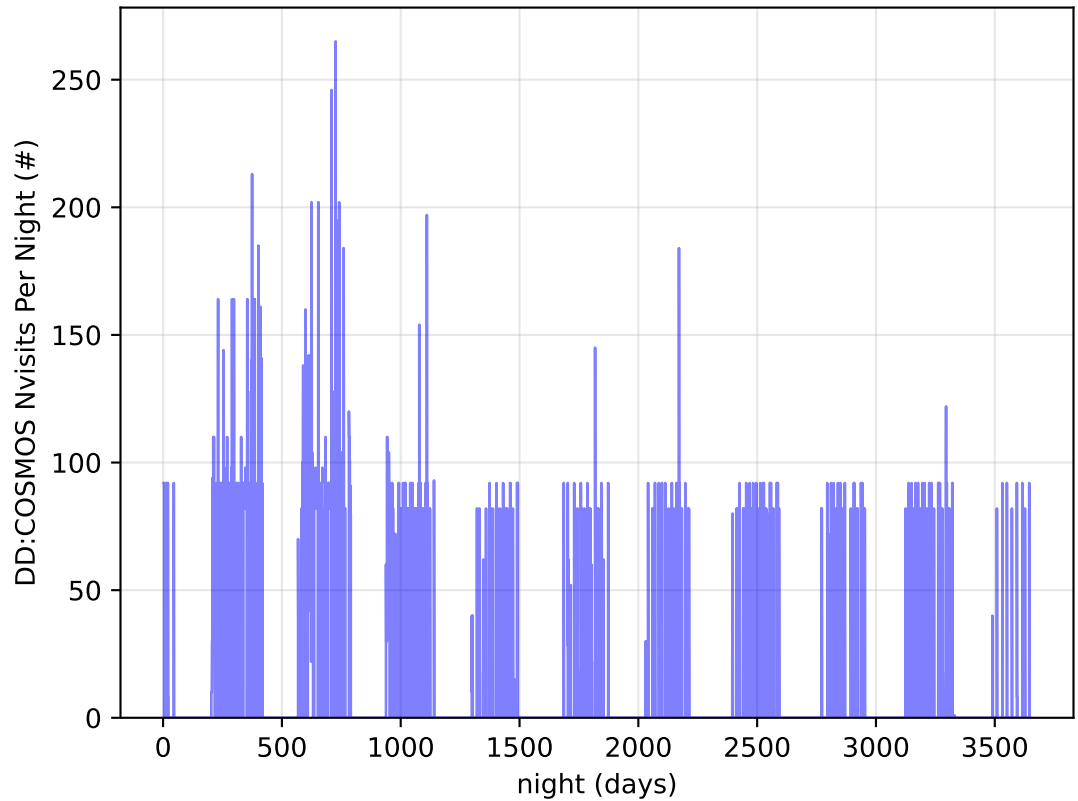
early_ss_template_fpextra1.5_v3.4_10yrs all bands: DD: COSMOS Nvisits Per Night
