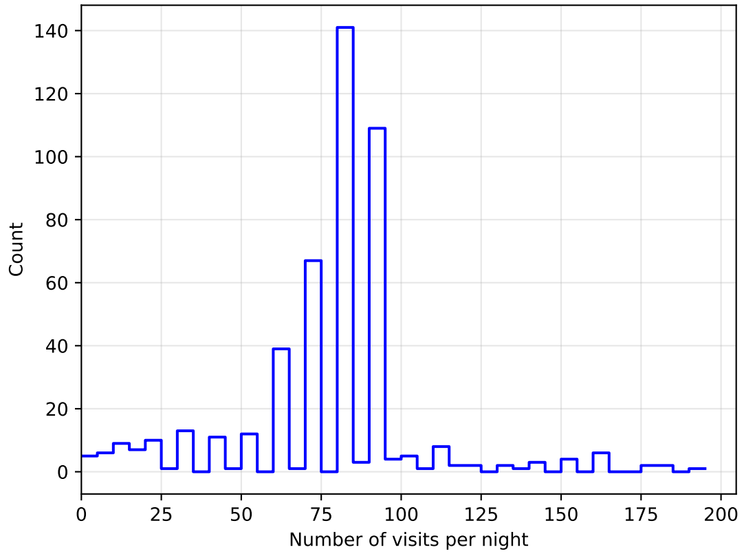
early_ss_template_fpextra1.5_v3.4_10yrs all bands: DD: COSMOS NVisitsPerNight
