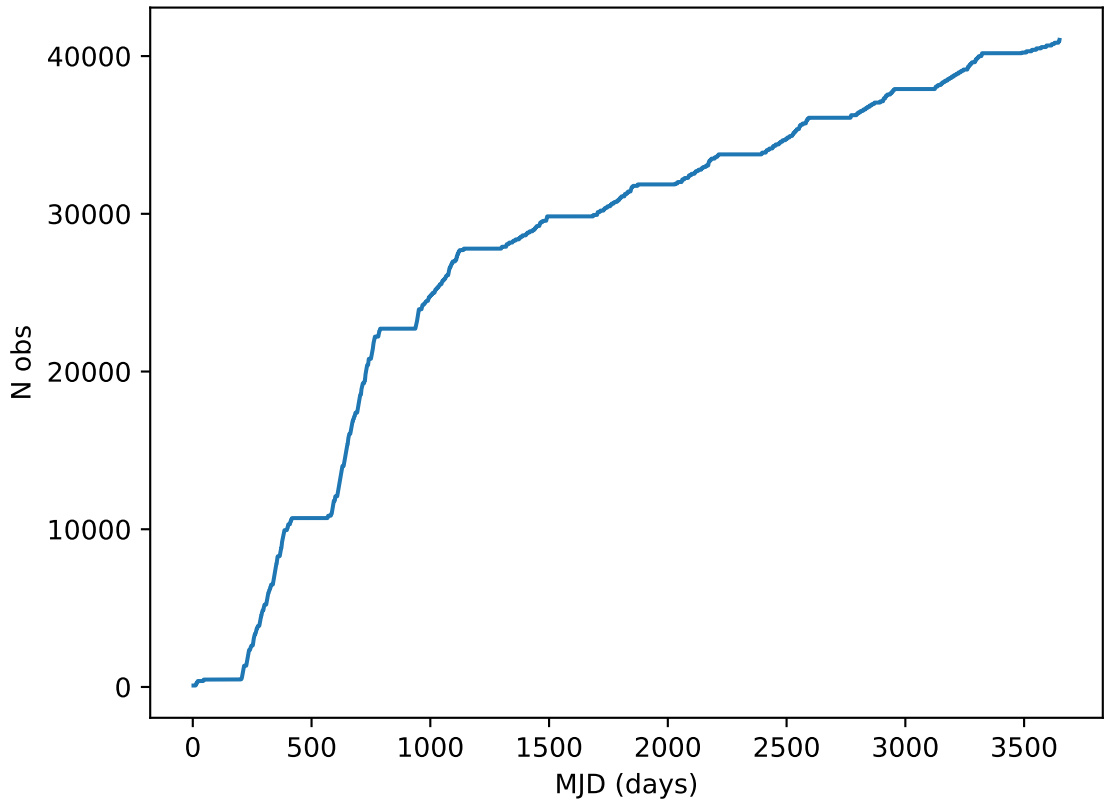
early_ss_template_fpextra1.5_v3.4_10yrs all bands: DD: COSMOS Cumulative NVisits
