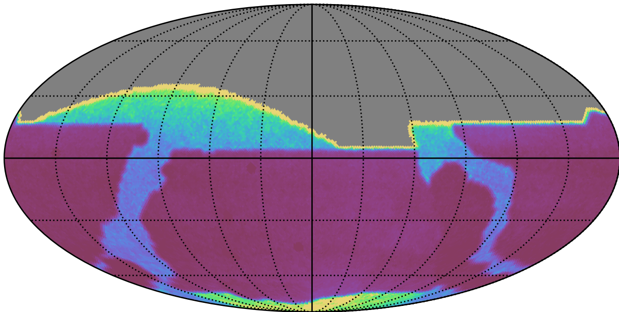
ddf_roll_deep_v3.5_10yrs : properMotion
