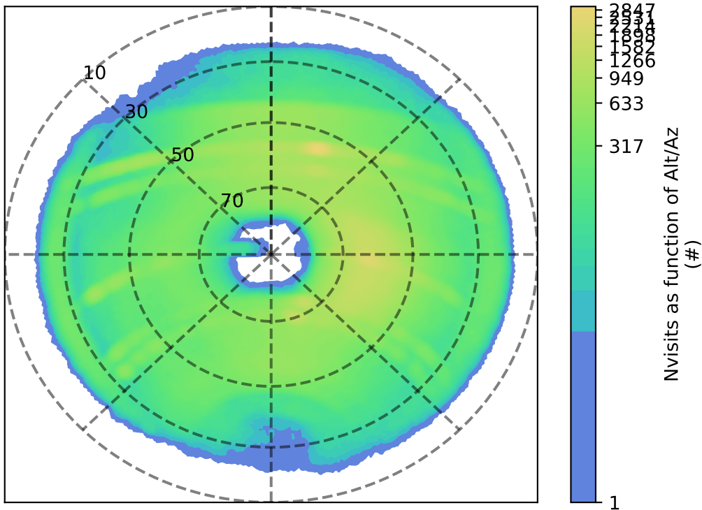
ddf_roll_deep_v3.5_10yrs z: Nvisits as function of Alt/Az
