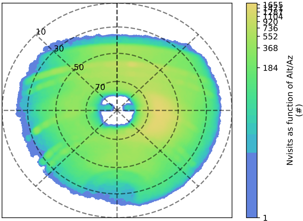
ddf_roll_deep_v3.5_10yrs y: Nvisits as function of Alt/Az
