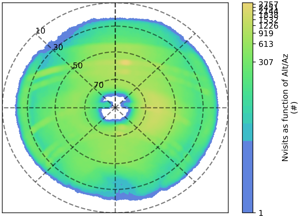
ddf_roll_deep_v3.5_10yrs r: Nvisits as function of Alt/Az
