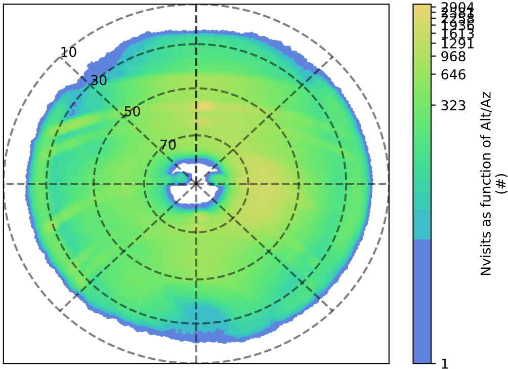
ddf_roll_deep_v3.5_10yrs i: Nvisits as function of Alt/Az
