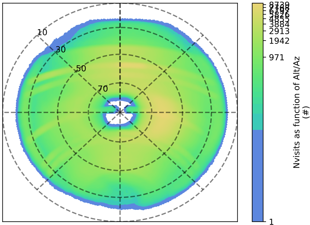
ddf_roll_deep_v3.5_10yrs : Nvisits as function of Alt/Az
