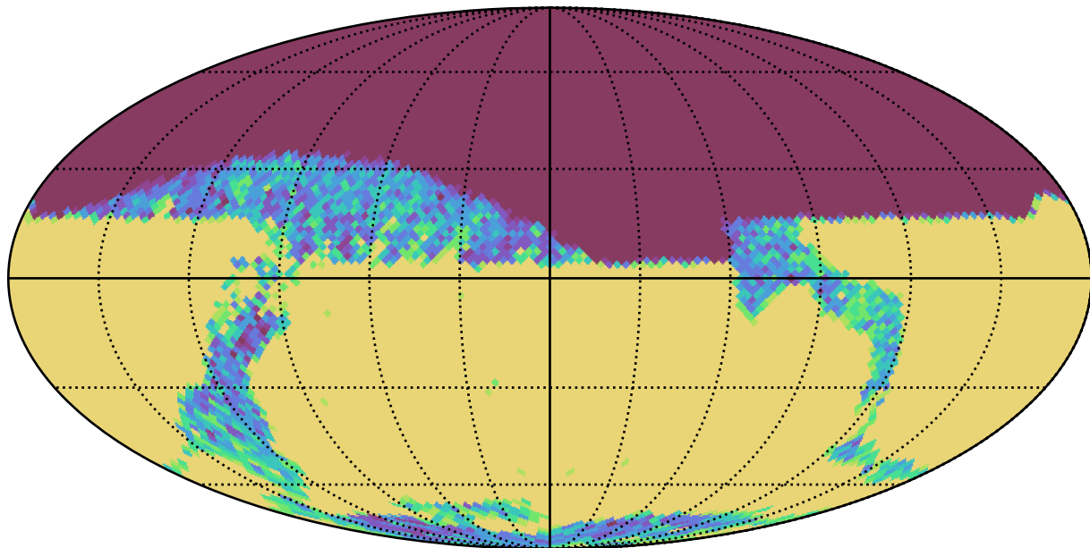
ddf_roll_deep_v3.5_10yrs z and night < 365: N year 1
